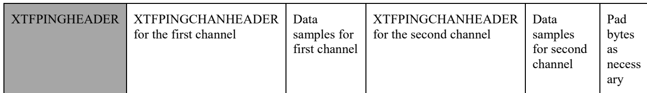
Figure 2. XTF Sonar Ping Header Data Layout (example for two-channel Sidescan)
