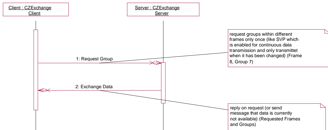
Figure 178: Sequence diagram
