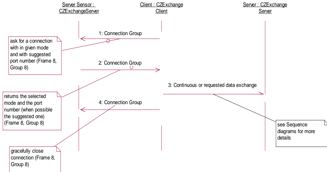
Figure 177: Create and shutdown connection to Exchange Server
