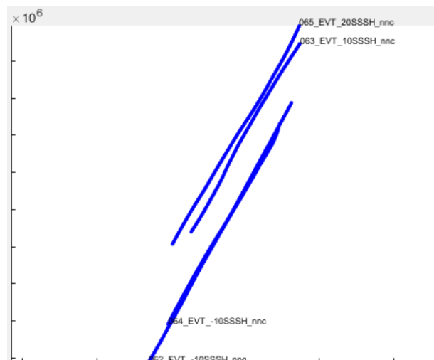
Figure 1 gMapPLDraw result
