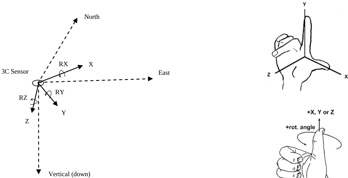
Figure shows multicomponent measurements and their respective rotation measurements relative to the reference system (north/east/vertical)
