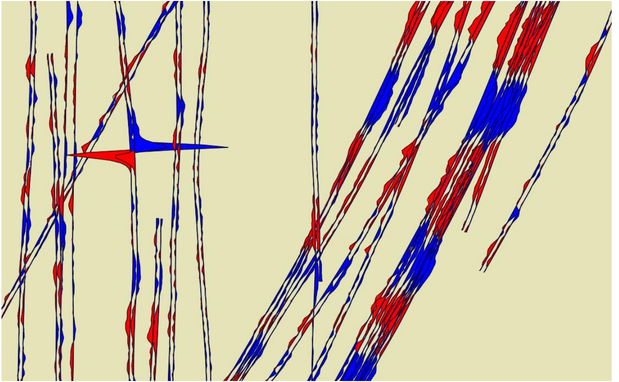
Figure 4 gAcadWiggleMask function result (script in AutoCad window); draw magnetic survey data along survey lines
